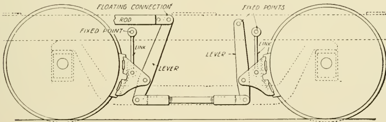
Fig. 80. Brake Mechanism, Showing Brake-Head, Shoes, and Hanger
